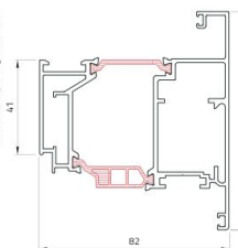
Anta Portoncino Ap. Esterna Outward Opening Door Leaf
