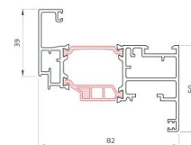
Anta Standard Standard Door Leaf
