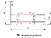
Telaio piano Full frame
