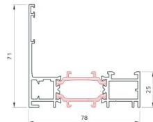
Telaio piano anta a scomparsa Retractable door full frame
