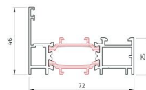
Telaio piano Flat frame
