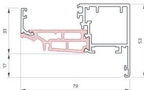
Anta Portoncino Ap. Interna Inner Opening Door Leaf
